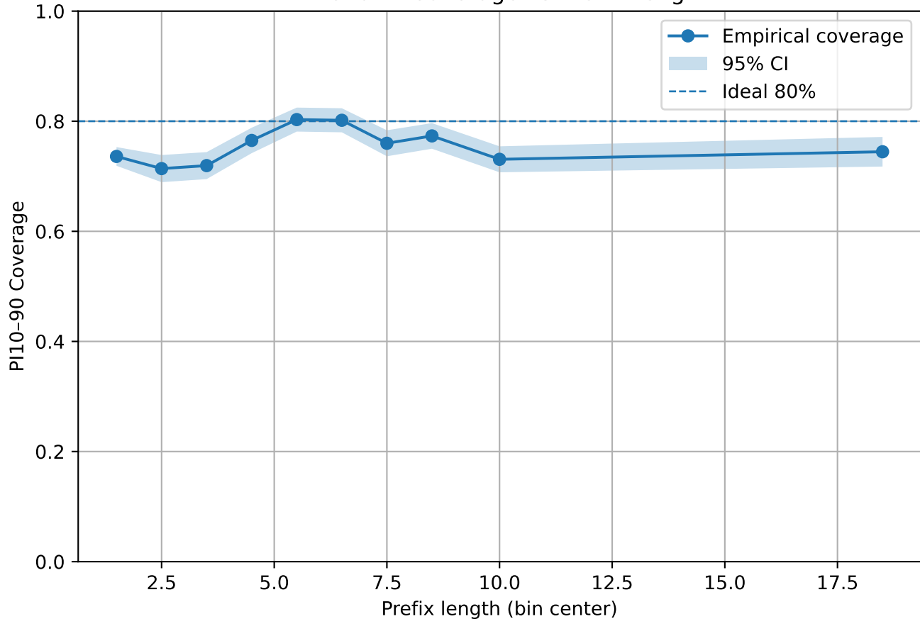
BPIC20ID: Coverage vs Prefix Length
